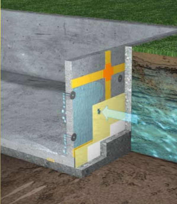
Leaks through damaged membrane are easily detected as water appears in the Sika® Control pipes and injection ports.
