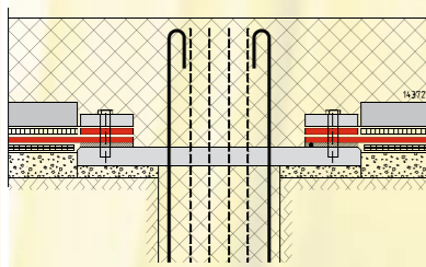
Details of the pile head
