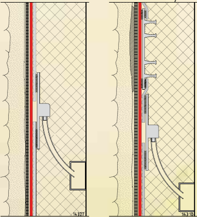
Sika® Control and injection ports
