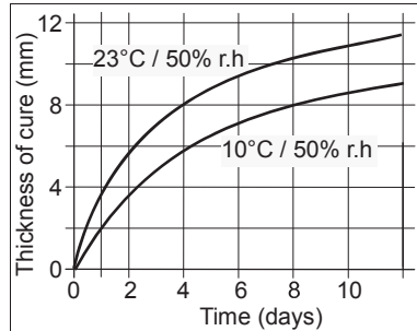
Diagram 1: Curing speed for Sikaflex®-265
